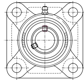
4 HOLE FLANGE
